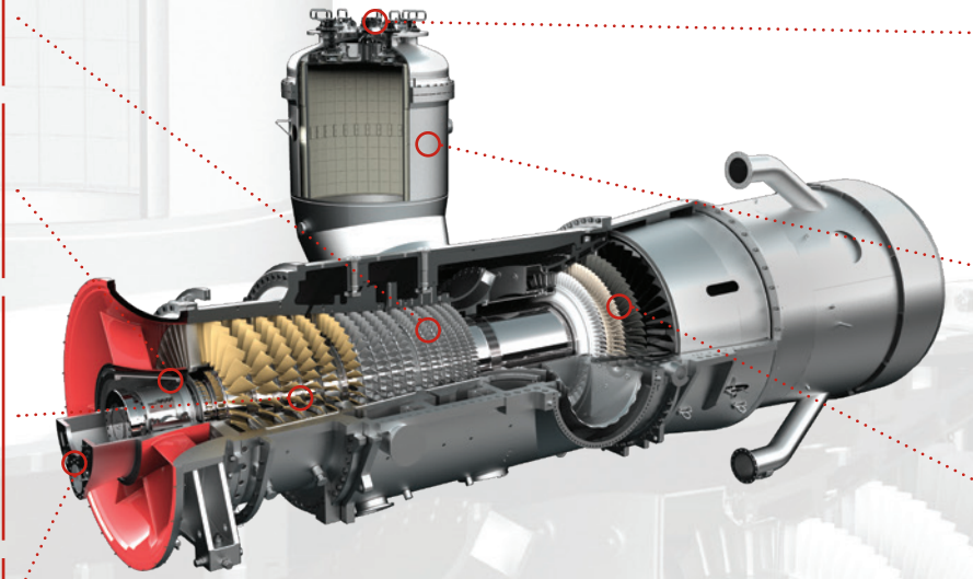
*All vanes and blades replaceable with rotor in place.
